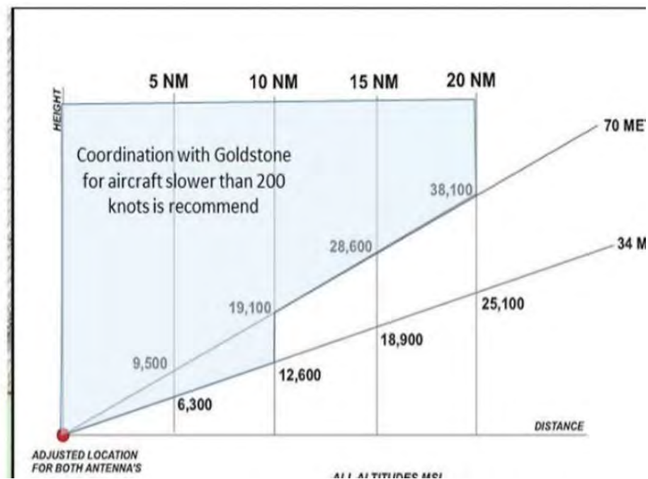
Figure 2-19: Goldstone Altitude Profiles
